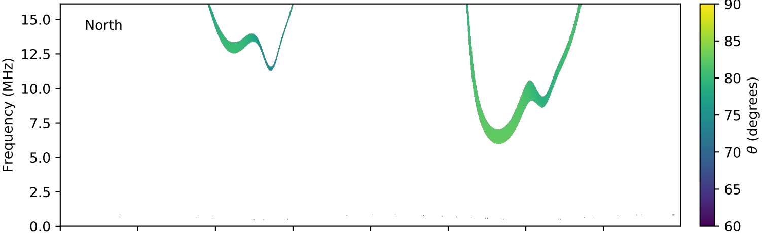
expres_cassini_jupiter_ganymede_isaac_lossc-wid1deg_3kev_20020324_v01.cdf
