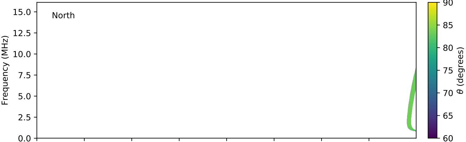
expres_cassini_jupiter_ganymede_isaac_lossc-wid1deg_3kev_20020321_v01.cdf
