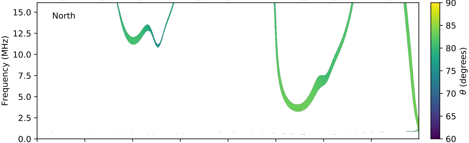
expres_cassini_jupiter_ganymede_isaac_lossc-wid1deg_3kev_20020317_v01.cdf
