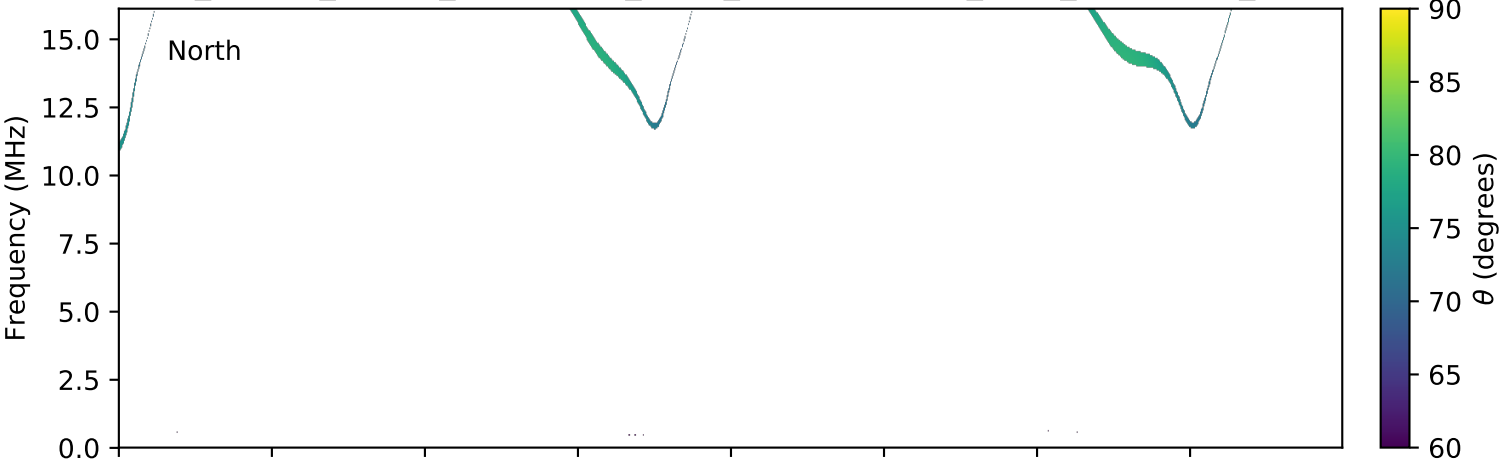
expres_cassini_jupiter_ganymede_isaac_lossc-wid1deg_3kev_20020316_v01.cdf
