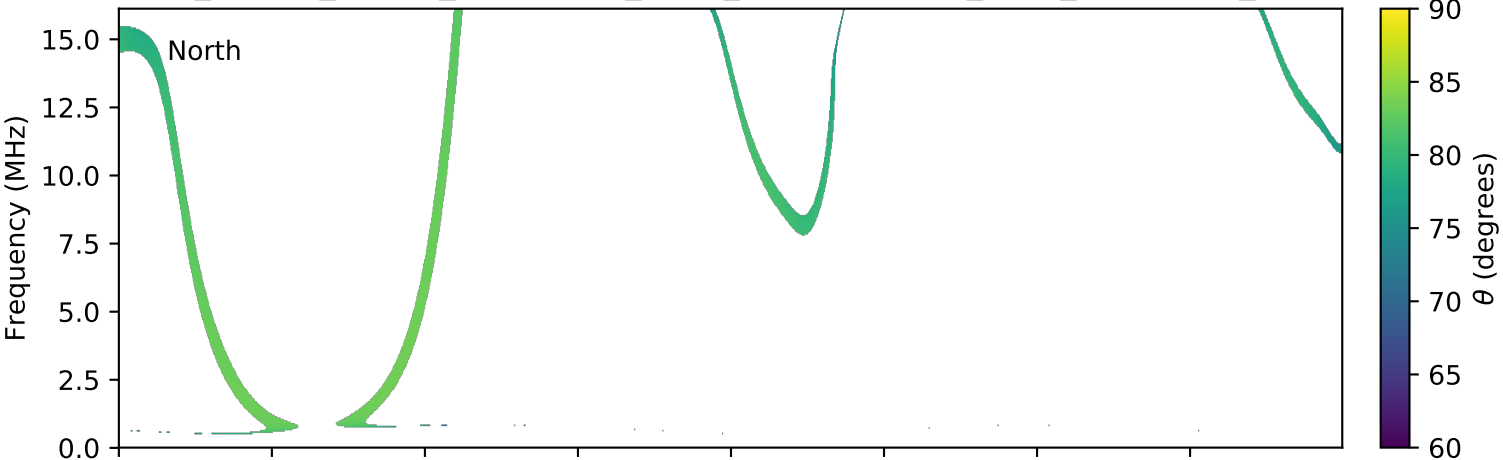
expres_cassini_jupiter_ganymede_isaac_lossc-wid1deg_3kev_20020315_v01.cdf
