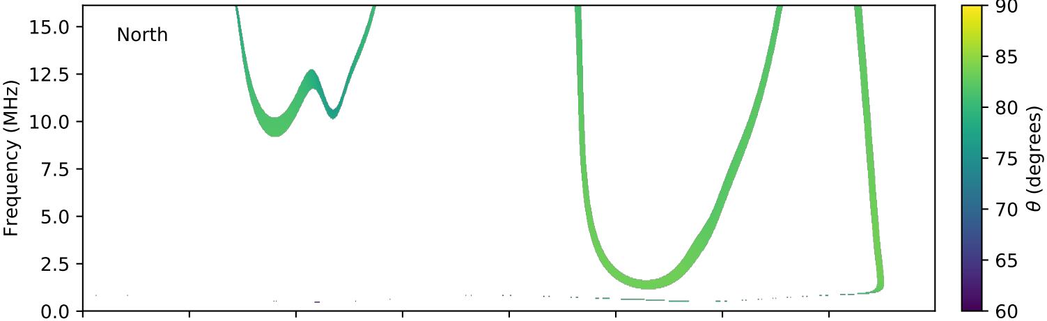
expres_cassini_jupiter_ganymede_isaac_lossc-wid1deg_3kev_20020310_v01.cdf
