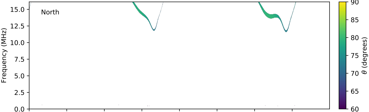
expres_cassini_jupiter_ganymede_isaac_lossc-wid1deg_3kev_20020309_v01.cdf
