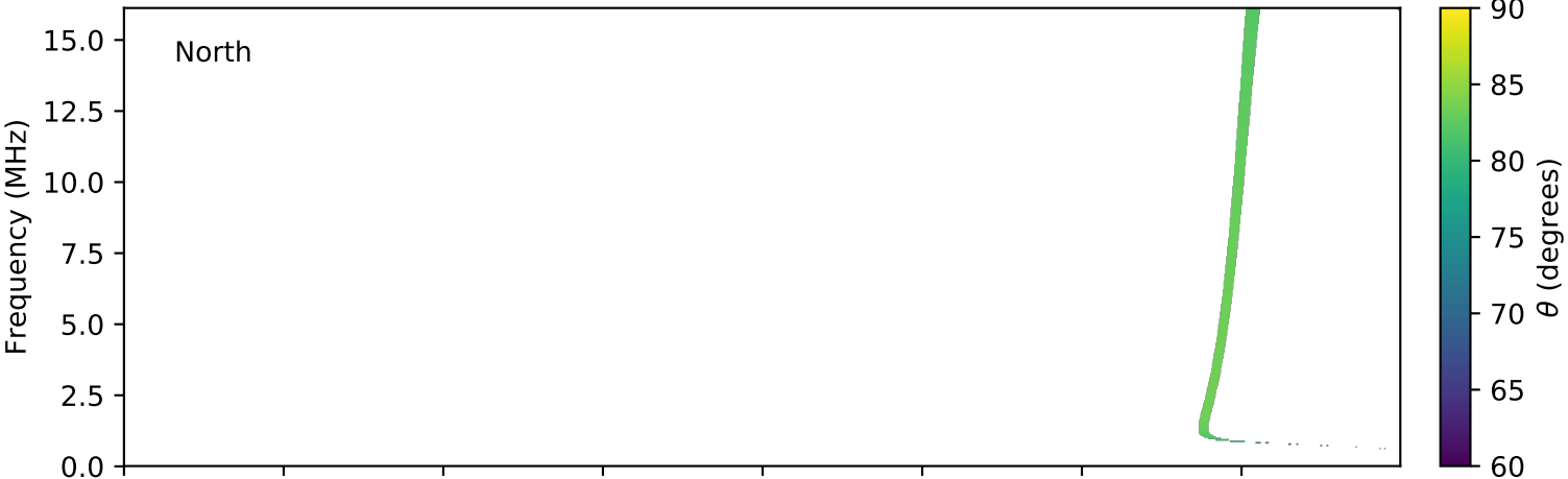
expres_cassini_jupiter_ganymede_isaac_lossc-wid1deg_3kev_20020307_v01.cdf
