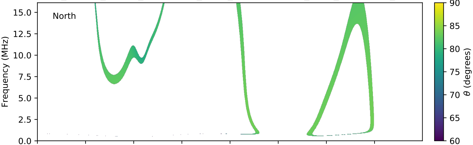
expres_cassini_jupiter_ganymede_isaac_lossc-wid1deg_3kev_20020303_v01.cdf
