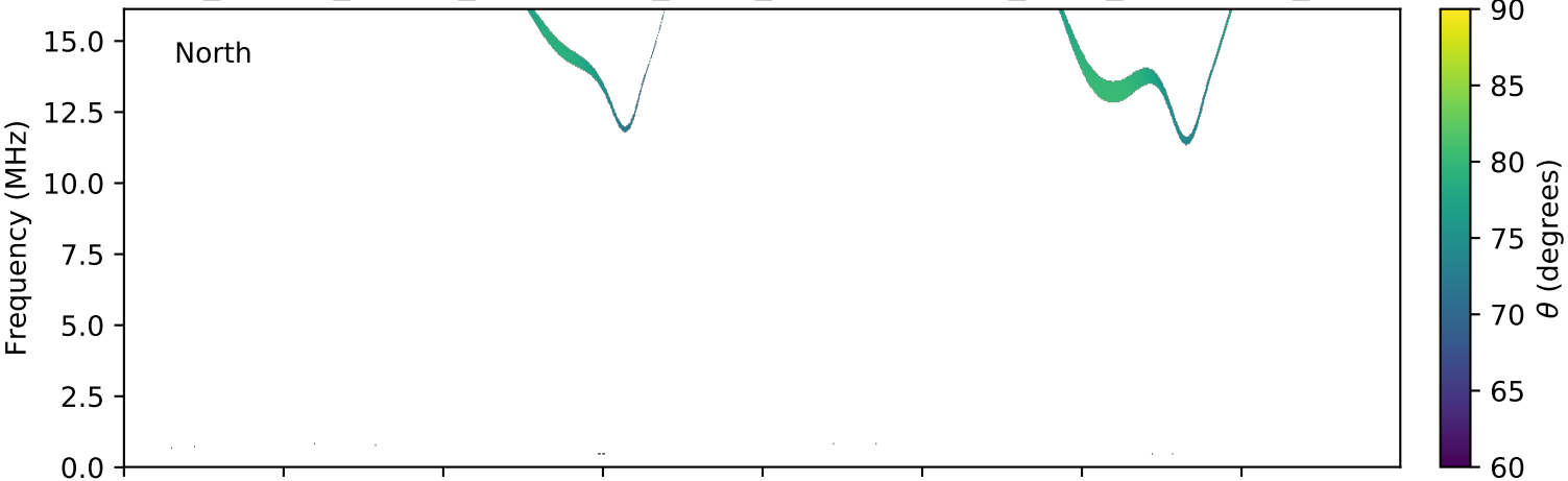
expres_cassini_jupiter_ganymede_isaac_lossc-wid1deg_3kev_20020302_v01.cdf
