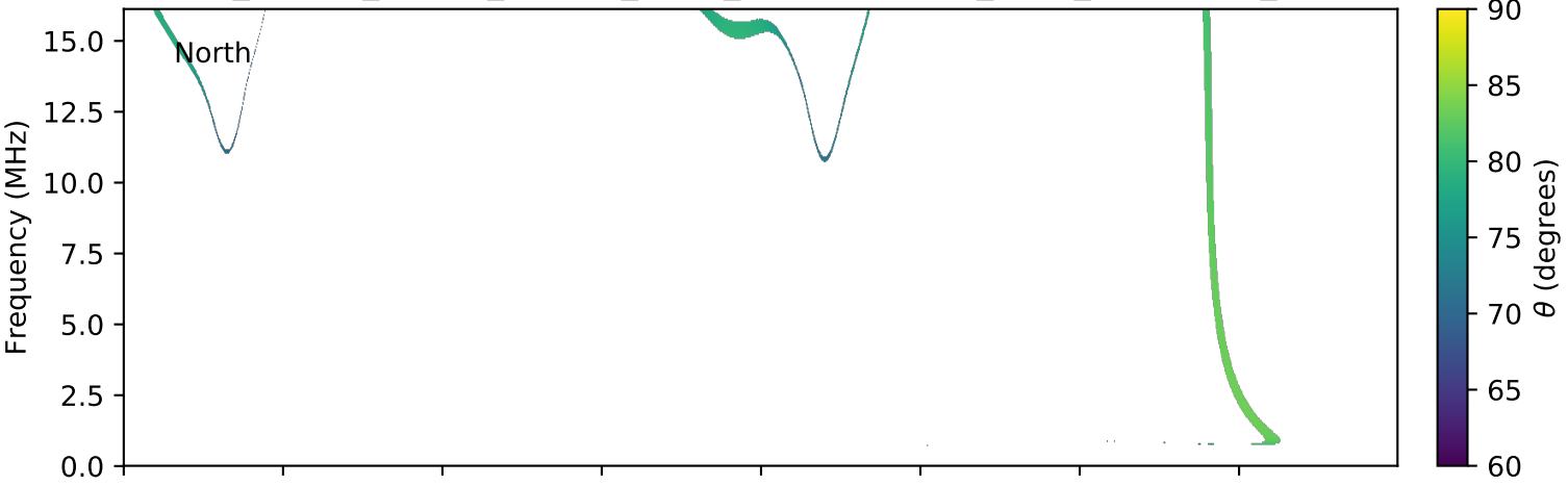
expres_cassini_jupiter_europa_isaac_lossc-wid1deg_3kev_20020330_v01.cdf
