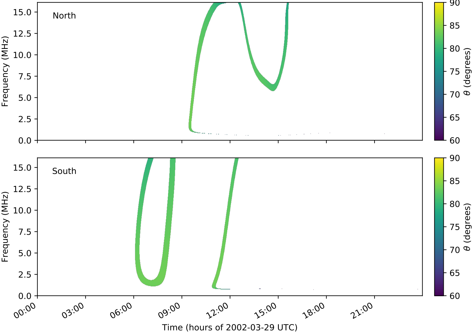
expres_cassini_jupiter_europa_isaac_lossc-wid1deg_3kev_20020329_v01.cdf
