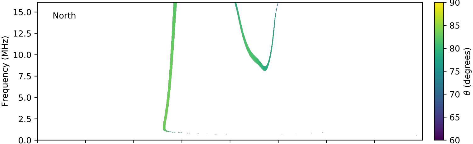
expres_cassini_jupiter_europa_isaac_lossc-wid1deg_3kev_20020322_v01.cdf
