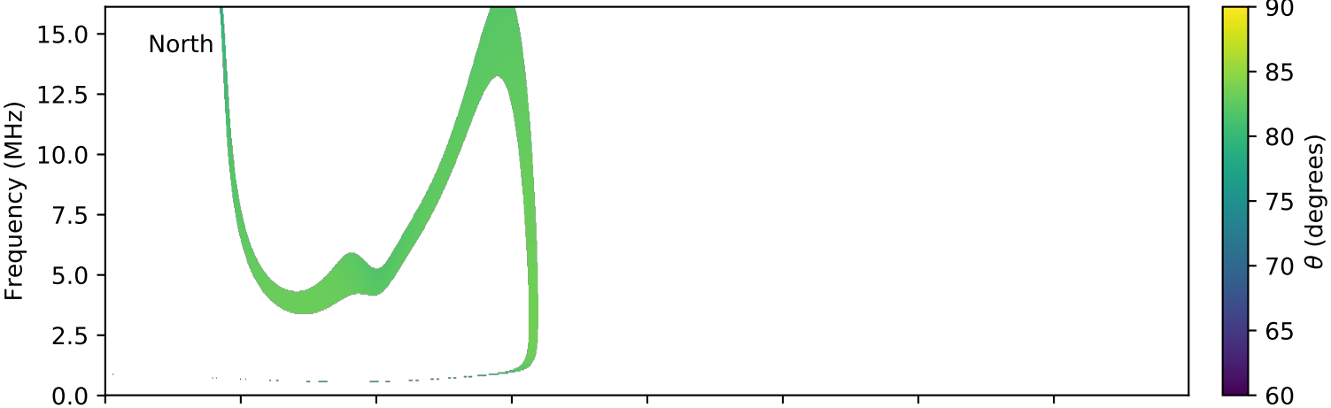
expres_cassini_jupiter_europa_isaac_lossc-wid1deg_3kev_20020320_v01.cdf
