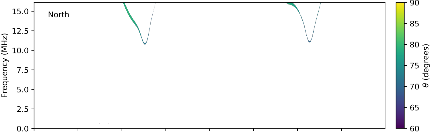
expres_cassini_jupiter_europa_isaac_lossc-wid1deg_3kev_20020319_v01.cdf
