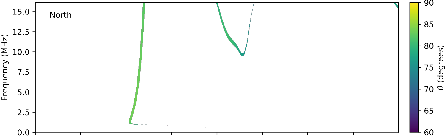
expres_cassini_jupiter_europa_isaac_lossc-wid1deg_3kev_20020315_v01.cdf
