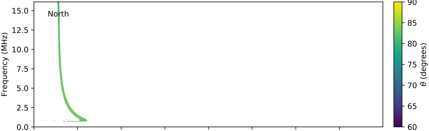
expres_cassini_jupiter_europa_isaac_lossc-wid1deg_3kev_20020313_v01.cdf
