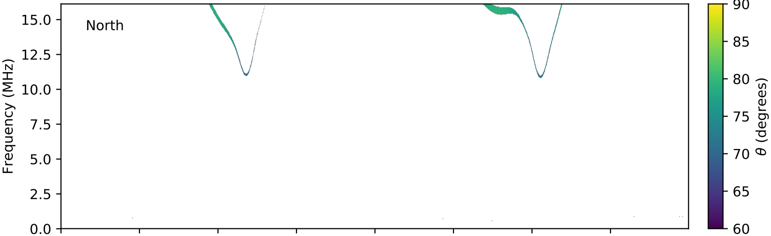
expres_cassini_jupiter_europa_isaac_lossc-wid1deg_3kev_20020312_v01.cdf
