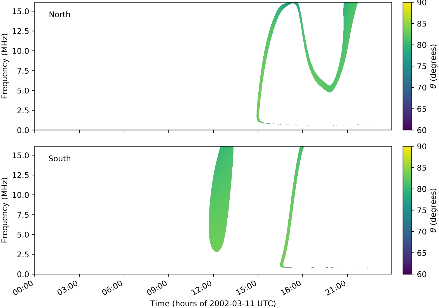
expres_cassini_jupiter_europa_isaac_lossc-wid1deg_3kev_20020311_v01.cdf
