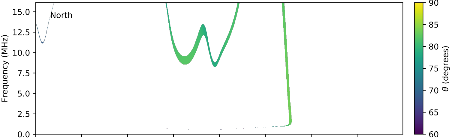
expres_cassini_jupiter_europa_isaac_lossc-wid1deg_3kev_20020309_v01.cdf
