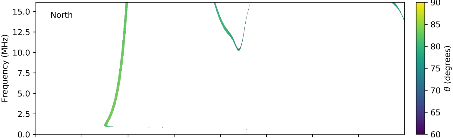
expres_cassini_jupiter_europa_isaac_lossc-wid1deg_3kev_20020308_v01.cdf
