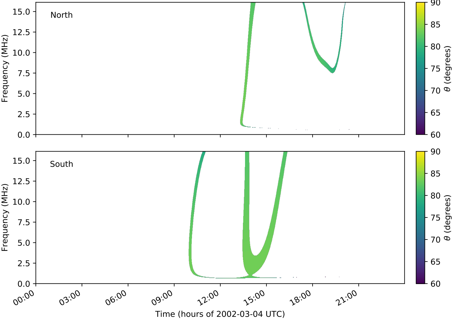
expres_cassini_jupiter_europa_isaac_lossc-wid1deg_3kev_20020304_v01.cdf
