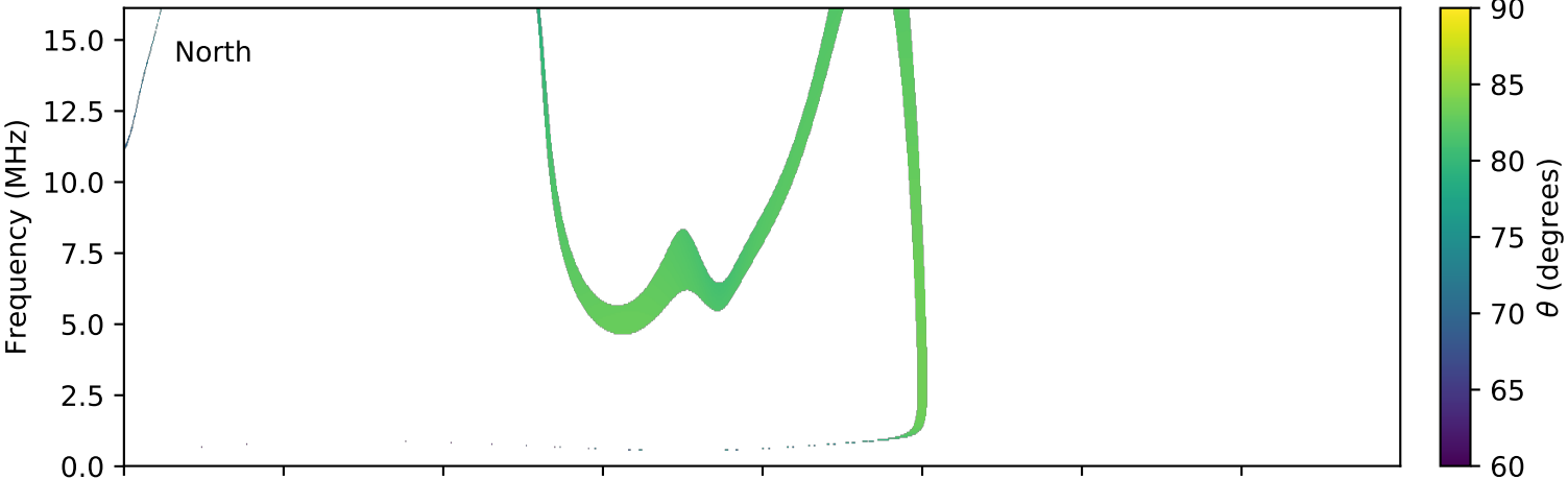
expres_cassini_jupiter_europa_isaac_lossc-wid1deg_3kev_20020302_v01.cdf
