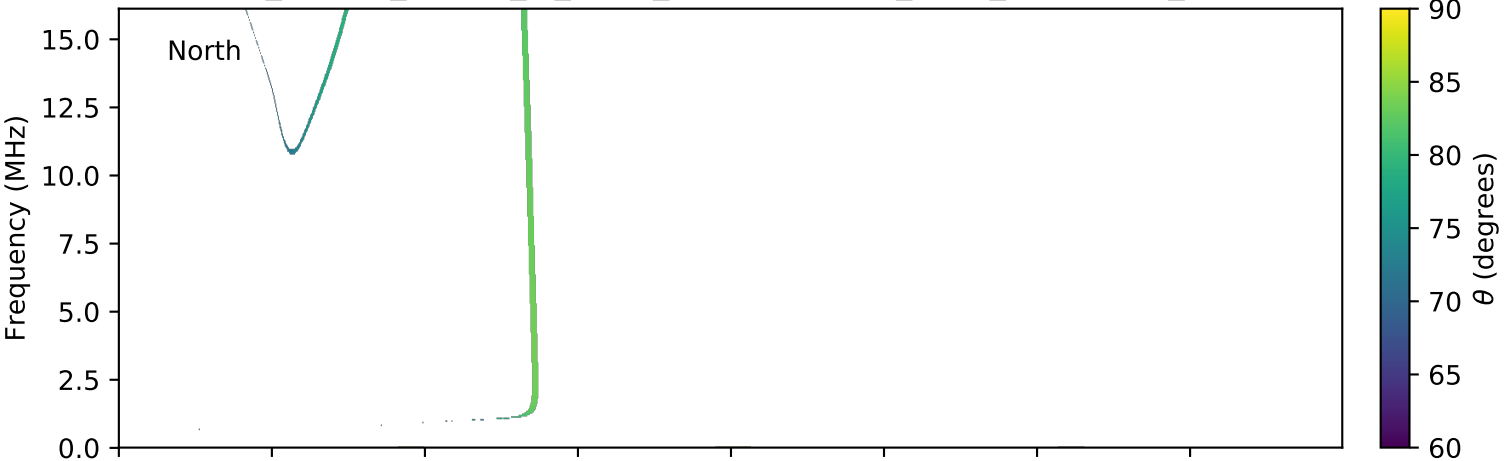
expres_cassini_jupiter_io_isaac_lossc-wid1deg_3kev_20020227_v01.cdf
