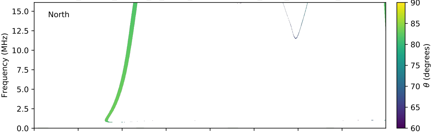
expres_cassini_jupiter_io_isaac_lossc-wid1deg_3kev_20020221_v01.cdf
