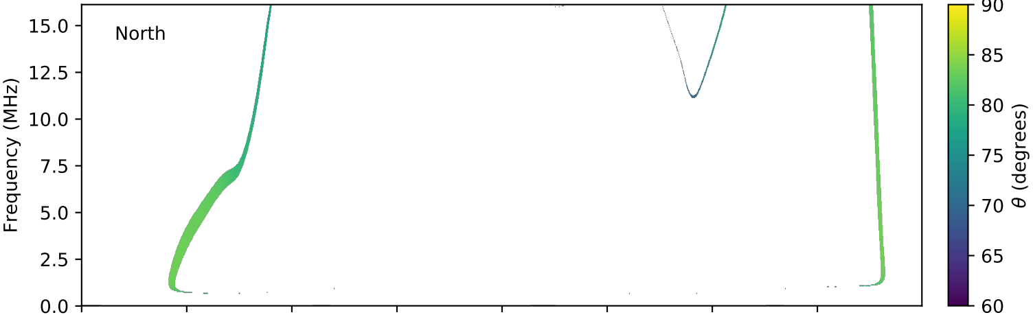
expres_cassini_jupiter_io_isaac_lossc-wid1deg_3kev_20020214_v01.cdf
