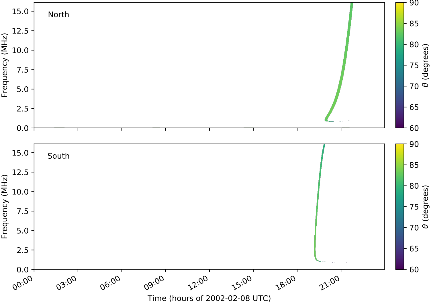
expres_cassini_jupiter_io_isaac_lossc-wid1deg_3kev_20020208_v01.cdf
