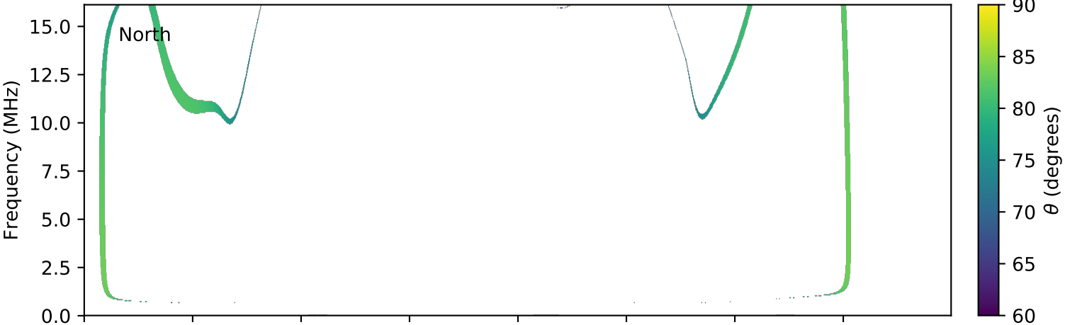
expres_cassini_jupiter_io_isaac_lossc-wid1deg_3kev_20020207_v01.cdf
