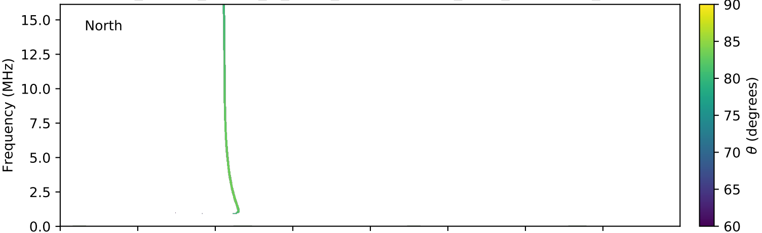
expres_cassini_jupiter_io_isaac_lossc-wid1deg_3kev_20020204_v01.cdf
