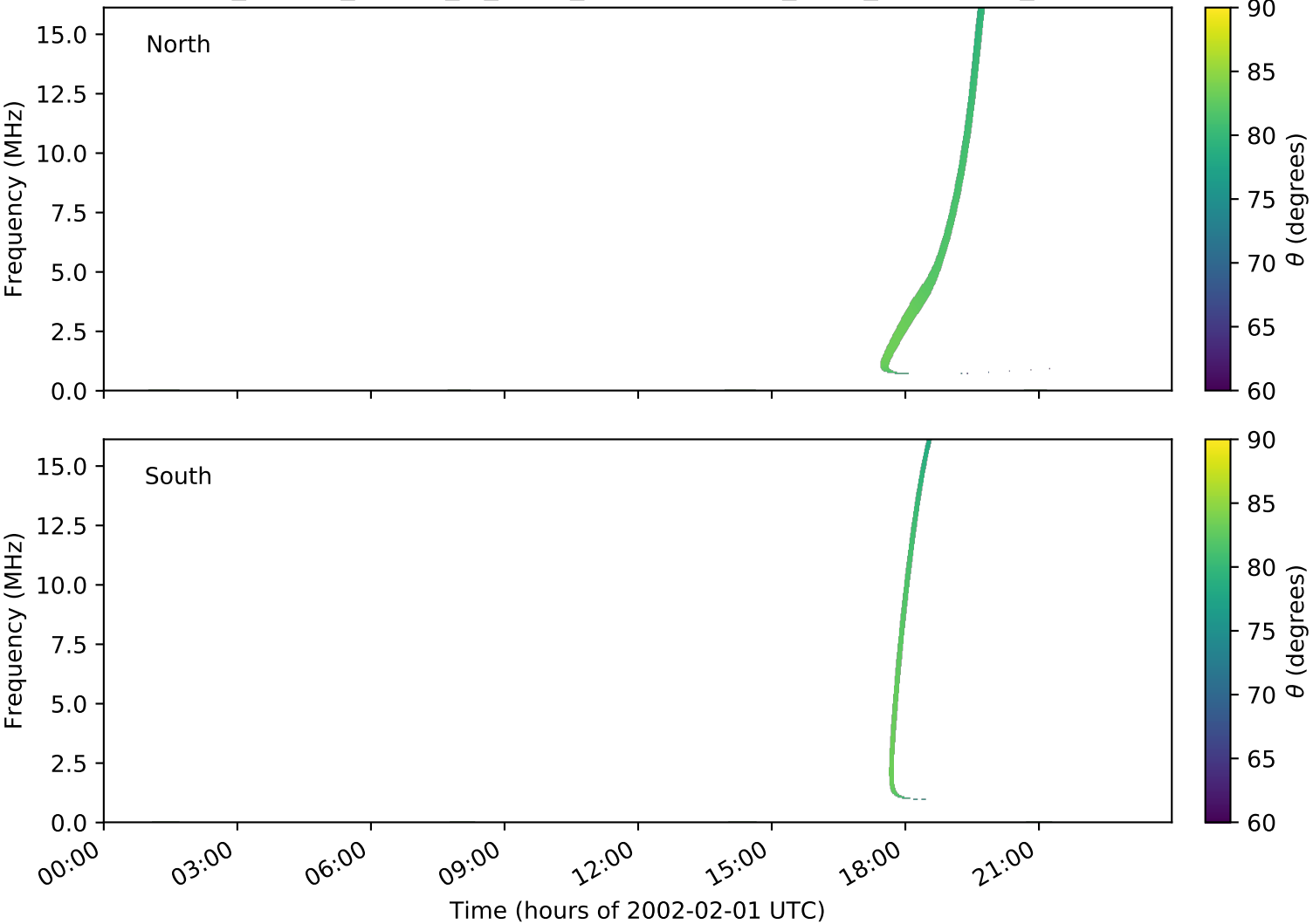
expres_cassini_jupiter_io_isaac_lossc-wid1deg_3kev_20020201_v01.cdf
