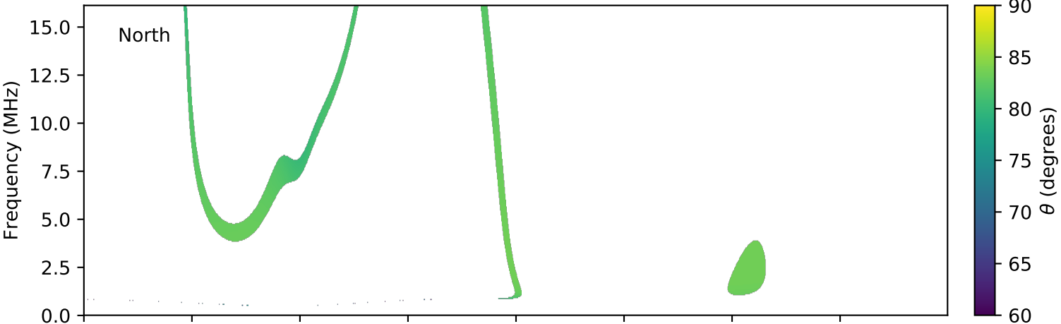
expres_cassini_jupiter_ganymede_isaac_lossc-wid1deg_3kev_20020224_v01.cdf
