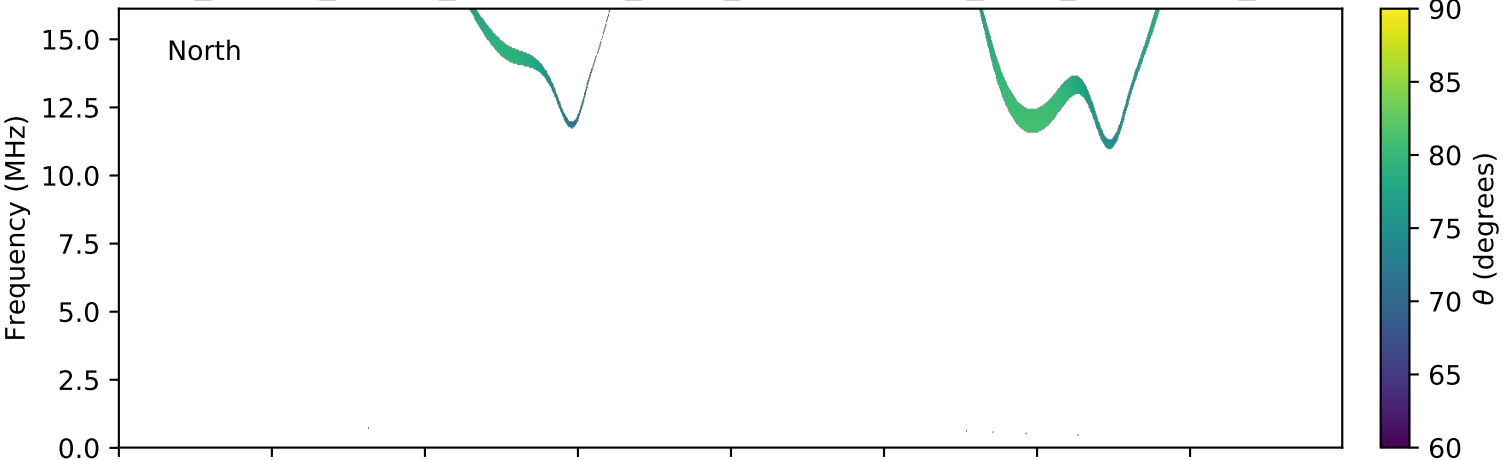
expres_cassini_jupiter_ganymede_isaac_lossc-wid1deg_3kev_20020223_v01.cdf
