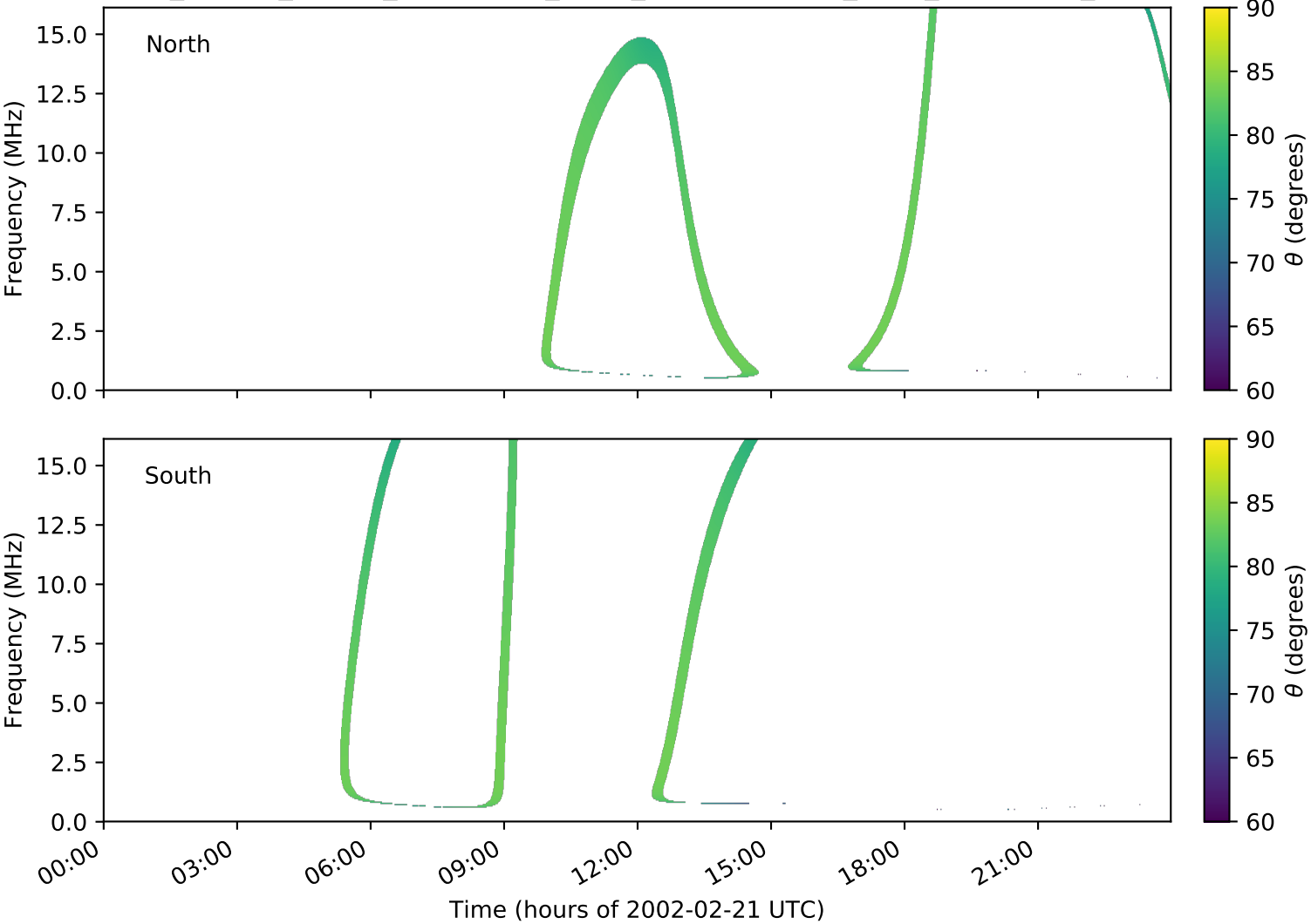
expres_cassini_jupiter_ganymede_isaac_lossc-wid1deg_3kev_20020221_v01.cdf
