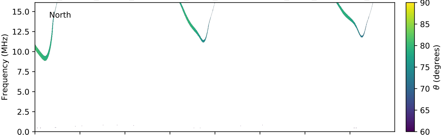
expres_cassini_jupiter_ganymede_isaac_lossc-wid1deg_3kev_20020215_v01.cdf
