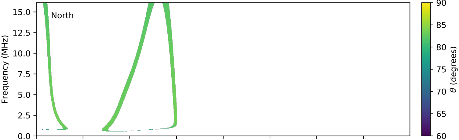
expres_cassini_jupiter_ganymede_isaac_lossc-wid1deg_3kev_20020210_v01.cdf
