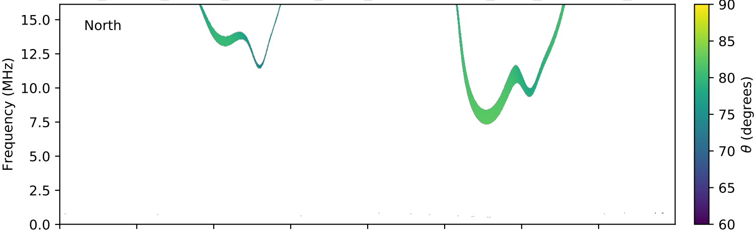
expres_cassini_jupiter_ganymede_isaac_lossc-wid1deg_3kev_20020209_v01.cdf
