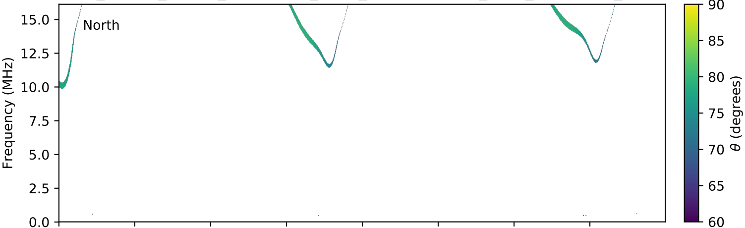
expres_cassini_jupiter_ganymede_isaac_lossc-wid1deg_3kev_20020208_v01.cdf
