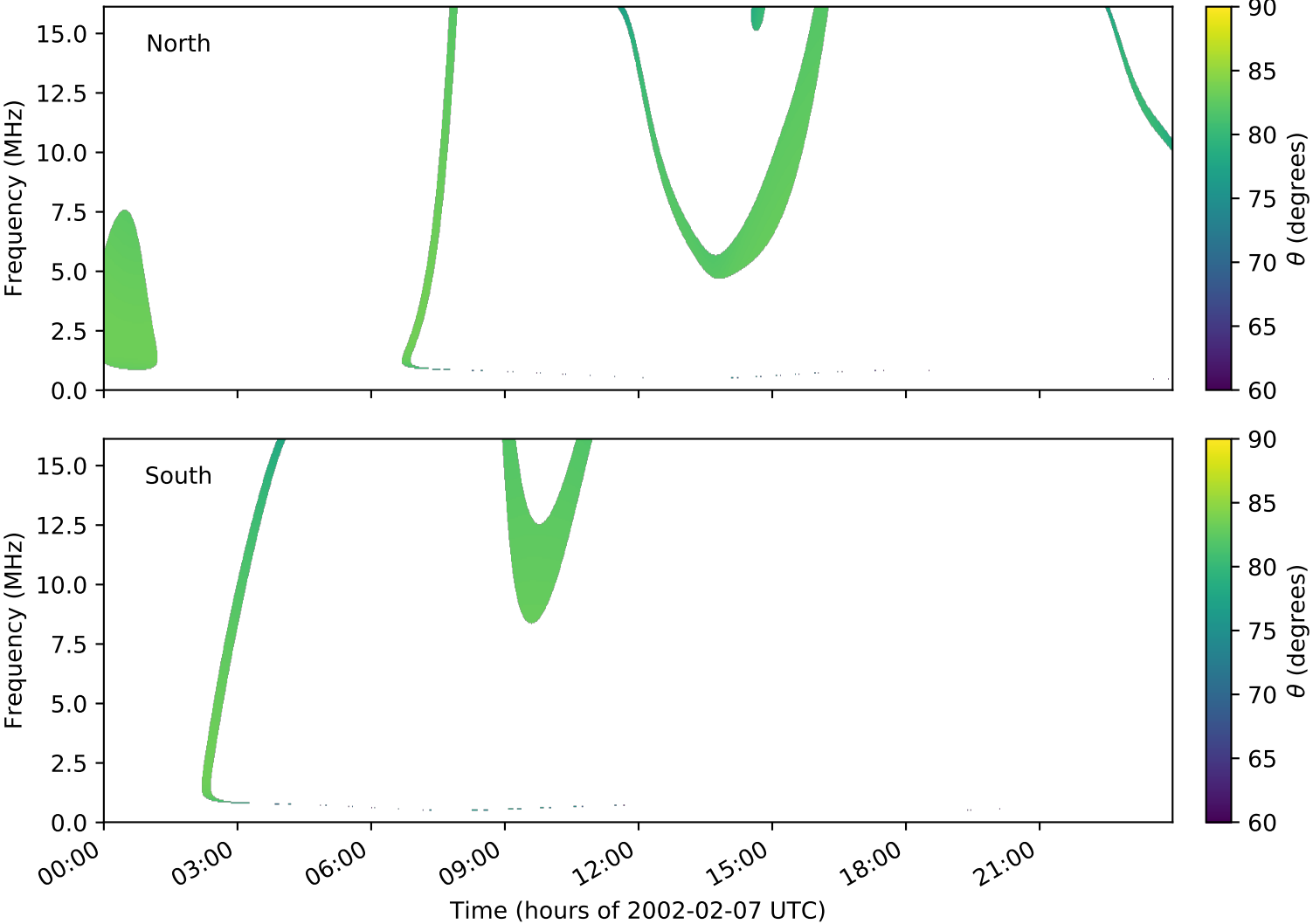
expres_cassini_jupiter_ganymede_isaac_lossc-wid1deg_3kev_20020207_v01.cdf
