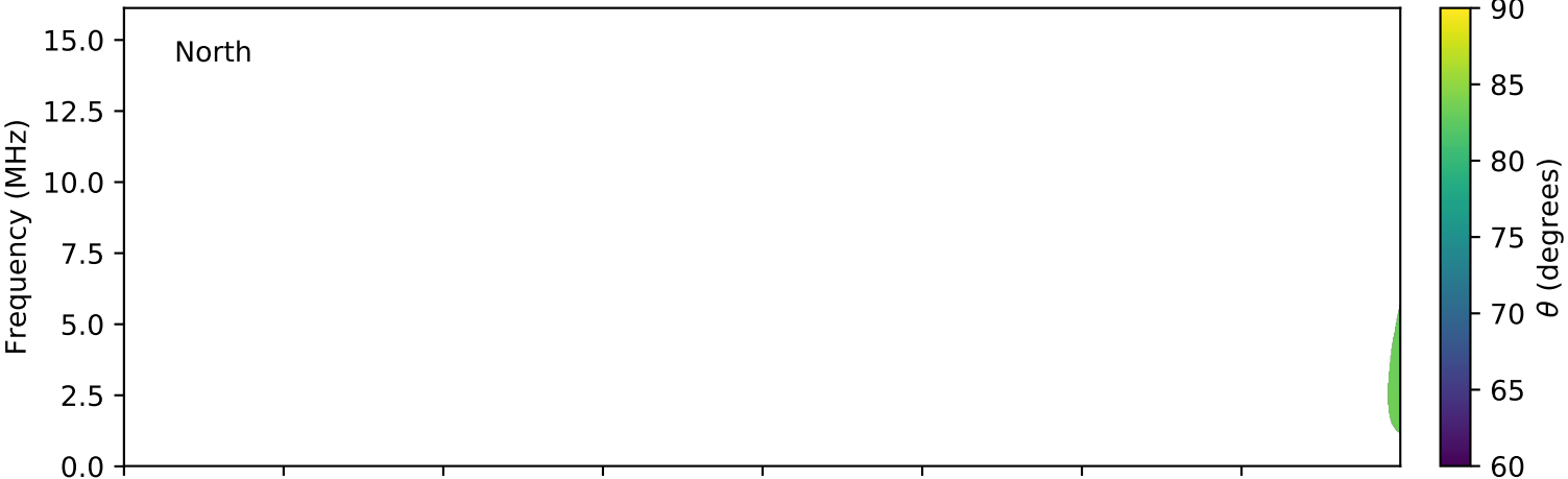
expres_cassini_jupiter_ganymede_isaac_lossc-wid1deg_3kev_20020206_v01.cdf
