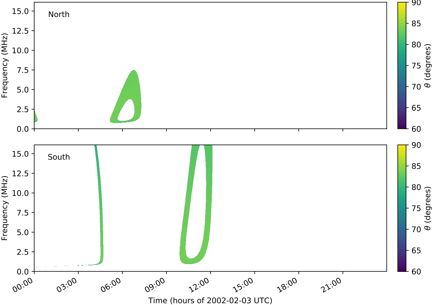
expres_cassini_jupiter_ganymede_isaac_lossc-wid1deg_3kev_20020203_v01.cdf
