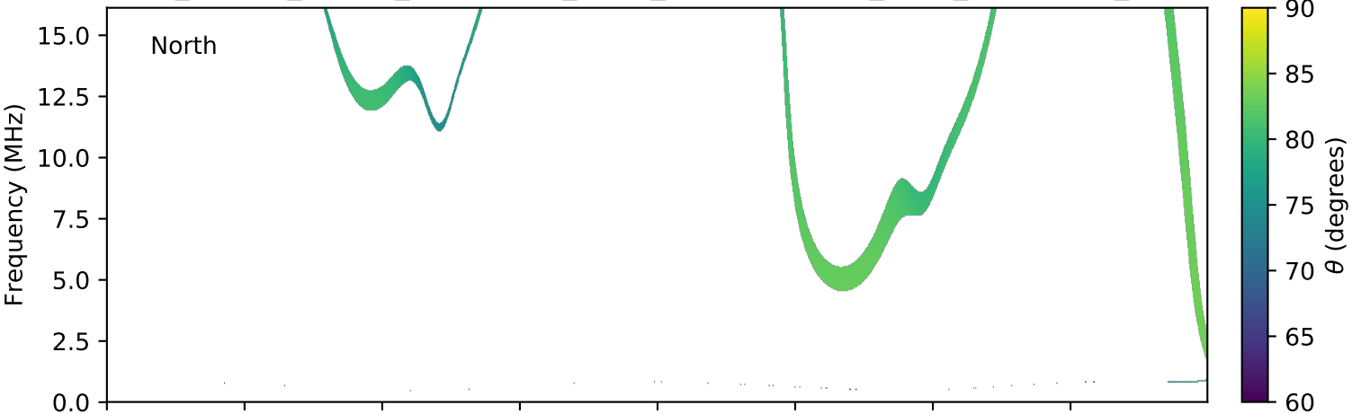
expres_cassini_jupiter_ganymede_isaac_lossc-wid1deg_3kev_20020202_v01.cdf
