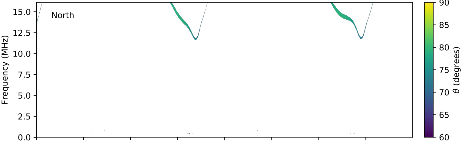
expres_cassini_jupiter_ganymede_isaac_lossc-wid1deg_3kev_20020201_v01.cdf
