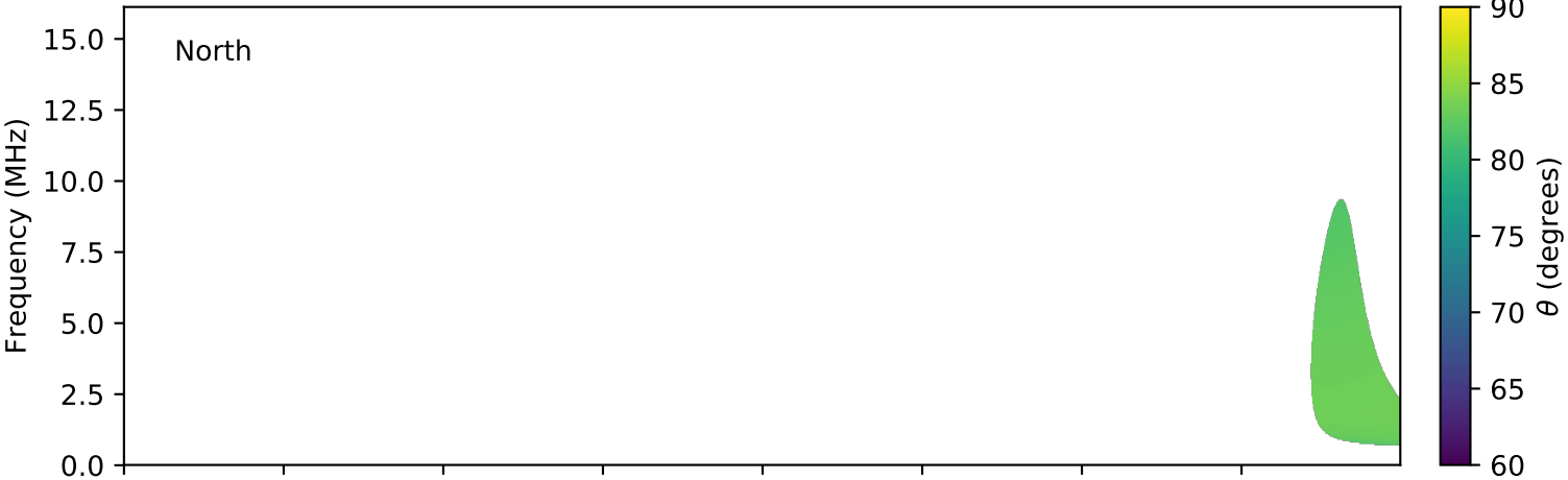
expres_cassini_jupiter_europa_isaac_lossc-wid1deg_3kev_20020228_v01.cdf
