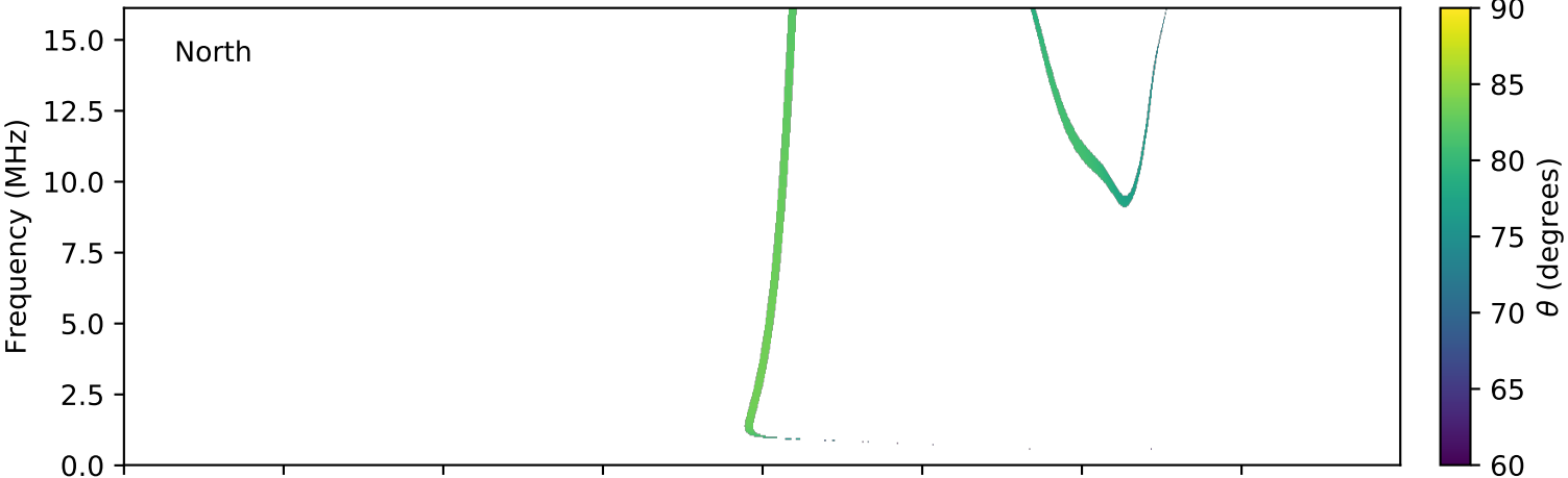
expres_cassini_jupiter_europa_isaac_lossc-wid1deg_3kev_20020225_v01.cdf
