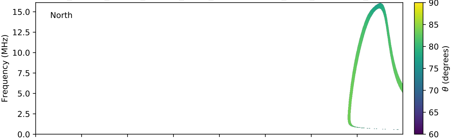
expres_cassini_jupiter_europa_isaac_lossc-wid1deg_3kev_20020221_v01.cdf
