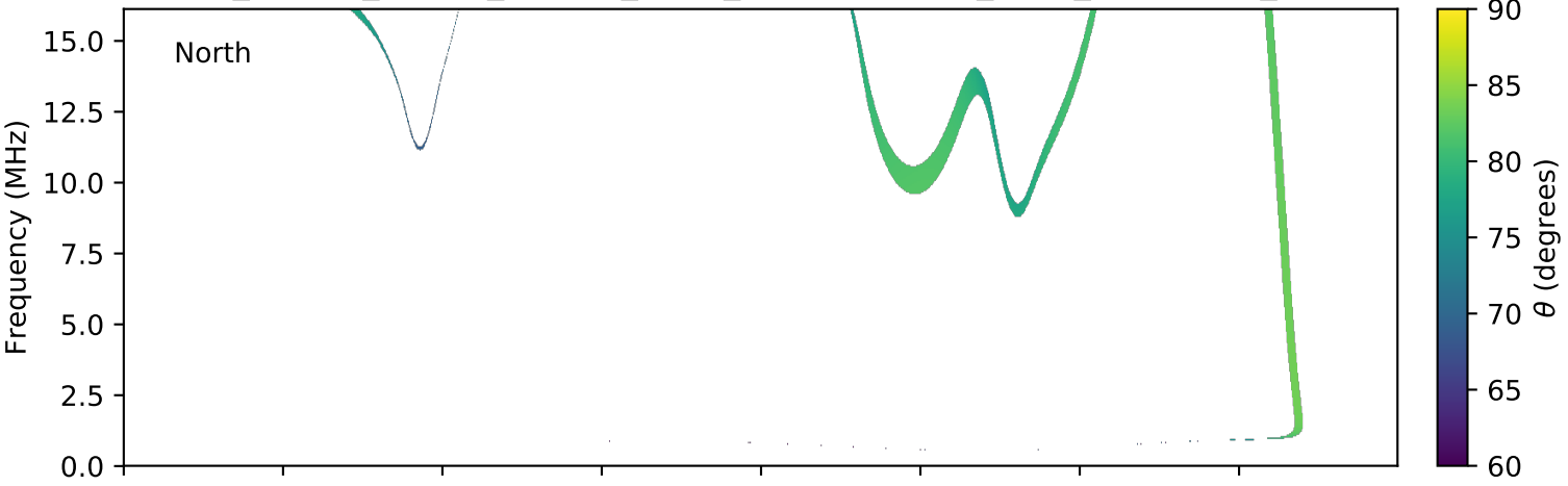
expres_cassini_jupiter_europa_isaac_lossc-wid1deg_3kev_20020219_v01.cdf
