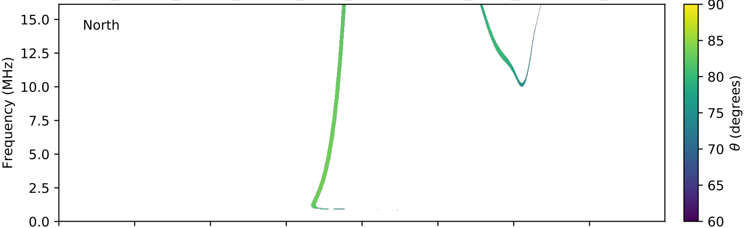
expres_cassini_jupiter_europa_isaac_lossc-wid1deg_3kev_20020218_v01.cdf
