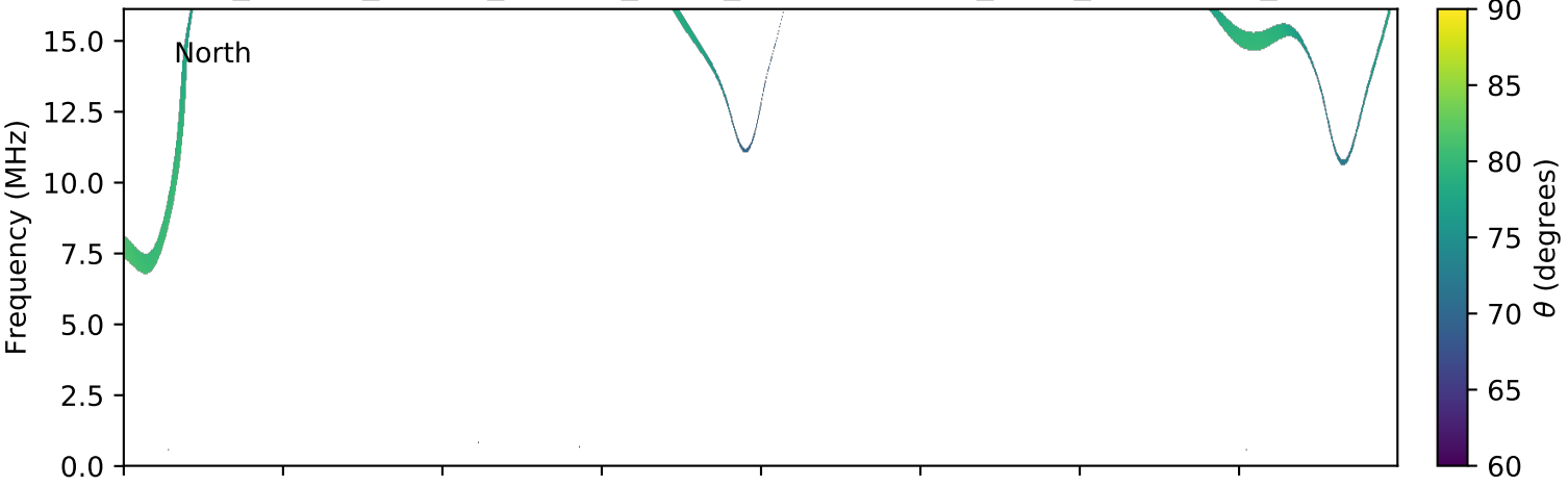
expres_cassini_jupiter_europa_isaac_lossc-wid1deg_3kev_20020215_v01.cdf
