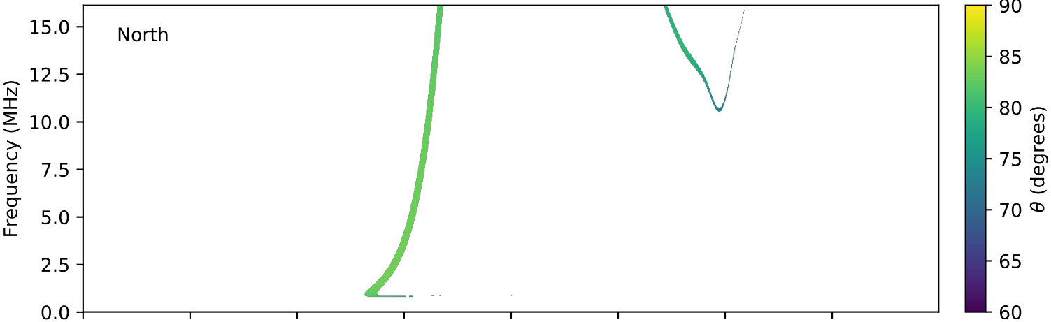
expres_cassini_jupiter_europa_isaac_lossc-wid1deg_3kev_20020211_v01.cdf
