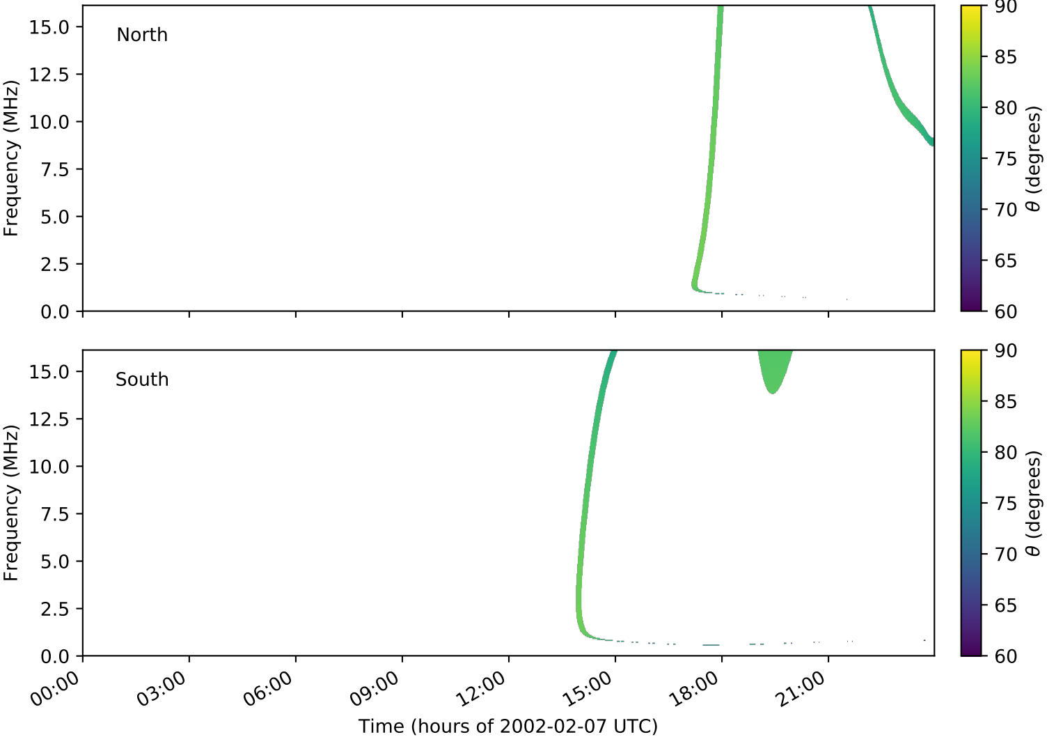
expres_cassini_jupiter_europa_isaac_lossc-wid1deg_3kev_20020207_v01.cdf
